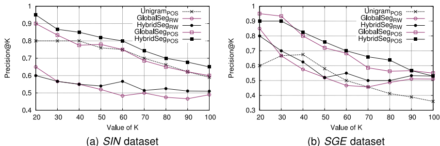
Fig. 8. Precision@K on two data sets.
