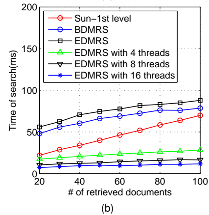
Fig. 7. The efficiency of a search with ten keywords of interest as input: (a) for the different sizes of document collection with the same dictionary, m = 4000 , and (b) for different numbers of retrieved documents with the same document collection and dictionary, n = 1000 , and m = 4000 .
